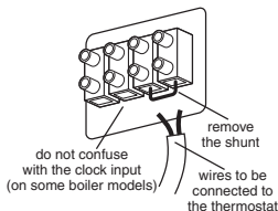
Example of a boiler terminal box
